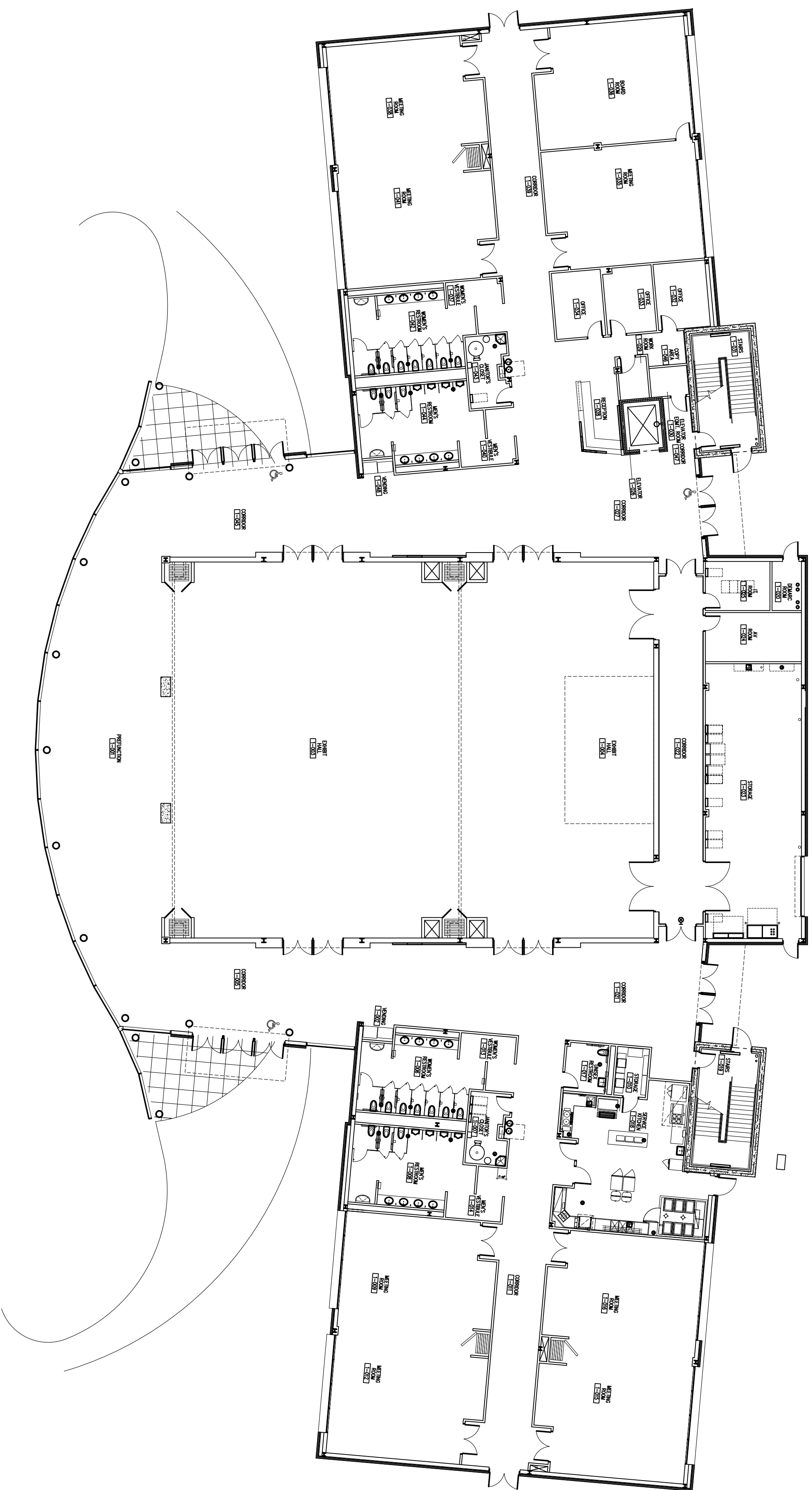
A FIRST FLOOR ARCHITECTURAL PLAN SCALE: 1/8" = 1'-0" 1/4" = 1'-0"
